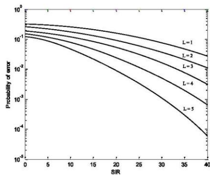
Figure 1. Probability of bit error versus SIR with the number of antenna elements L as a variable and the number of interferer N_i is equal to 10.
